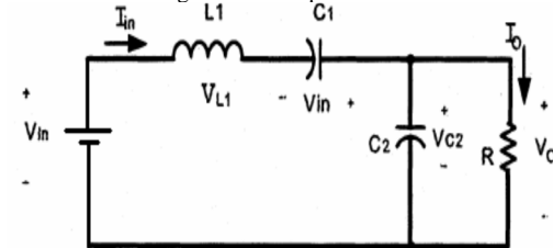
Figure. 5 Mode 2 operation
