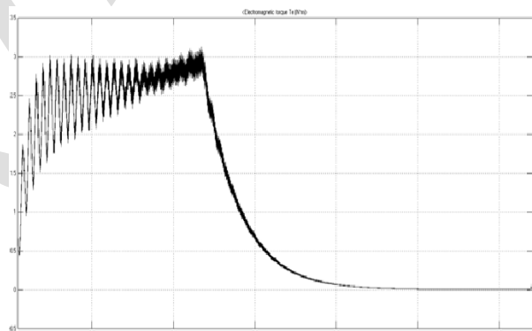
Figure.11 Electromagnetic Torque
