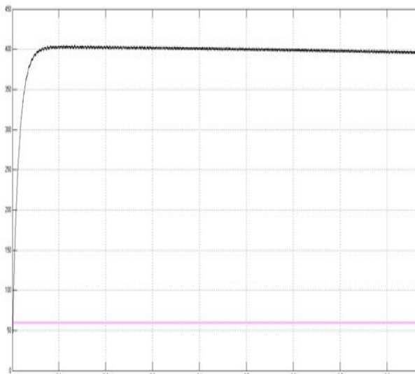
Figure.8 Input and Output Voltage of Positive Output Super-lift Luo Converter
