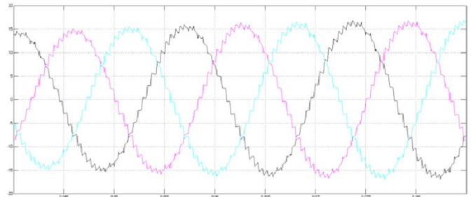
Figure.9 Stator Current of Three phase Induction Motor
