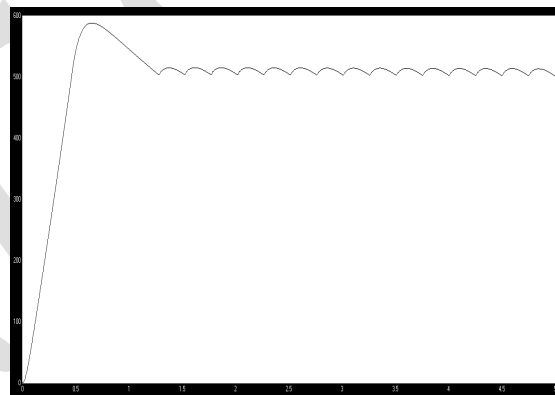
Figure.10 Speed Response of Three phase Induction Motor
