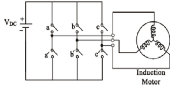
Figure. 1: Power circuit of induction motor
