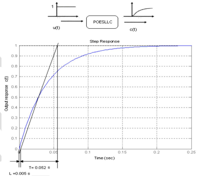
Figure.6 S- shaped curve of step response of Positive output elementary super lift Luo converter
